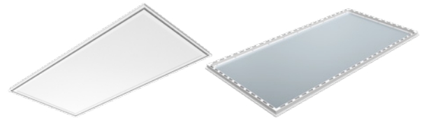
LPANA0612ND Up To 49W L 1195mm x W 595mm x H 25mm
