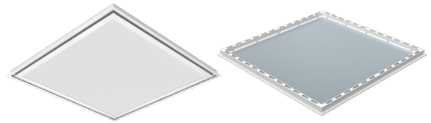
LPANA0606ND Up To 40W L 595mm x W 595mm x H 25mm
