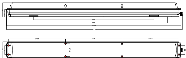
4FT 60/50/40/35W L 1170mm x W 110mm x D 95mm
