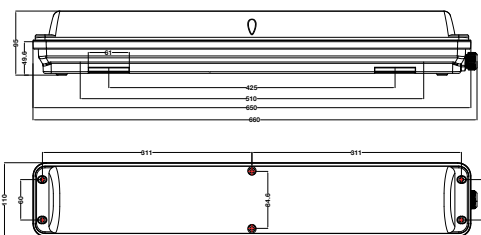
2FT 30/25/20/15W L 660mm x W 110mm x D 95mm
