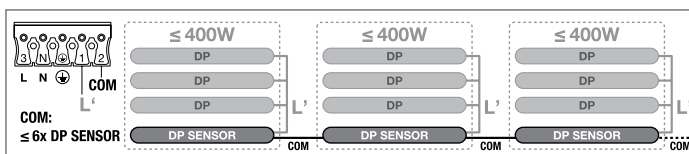
Bedrading leader/follower en leader/leader
