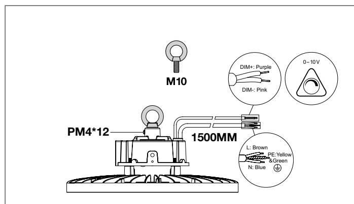
HIGH BAY 150W 4000K 110° ML
