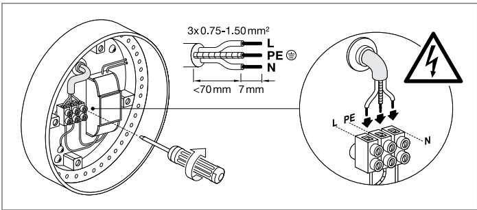
ENDURA STYLE RING
