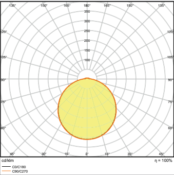
SURFACE COMPACT IK10 300 24W 4000K IP65
