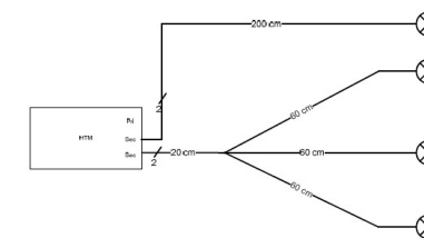
Parallel Circuit
