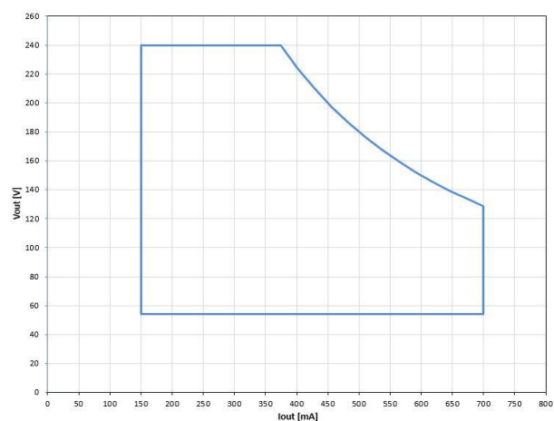
Typical Operating window
