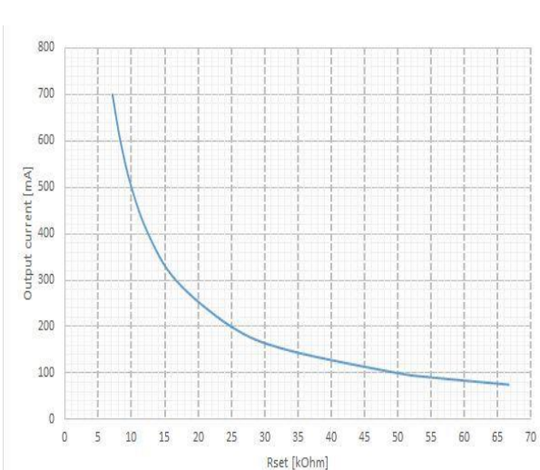
Typical Iout vs Rset
