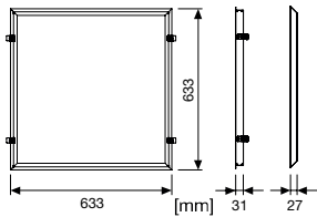
PL 600 E SUSPENSION KIT
