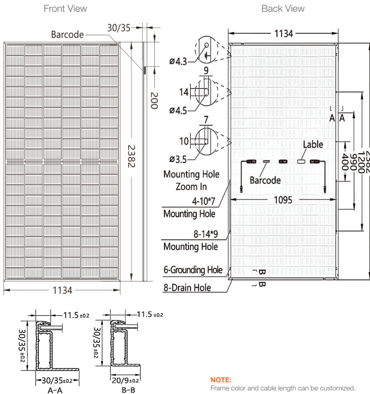
Dimensions of PV module (mm)
