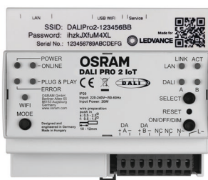
OSRAM DALI PRO 2 IOT LDV EAN-code: 4052899 627079
