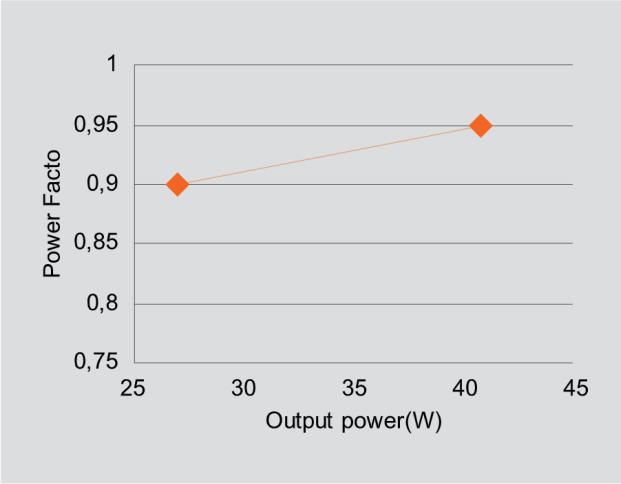
40W 900mA POWER FACTOR
