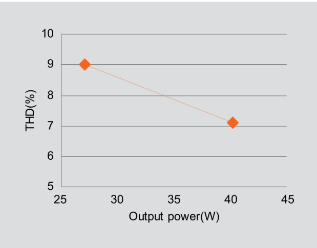
40W 900mA THD
