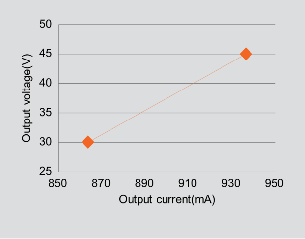
40W 900mA TYPICAL OPERATING WINDOW
