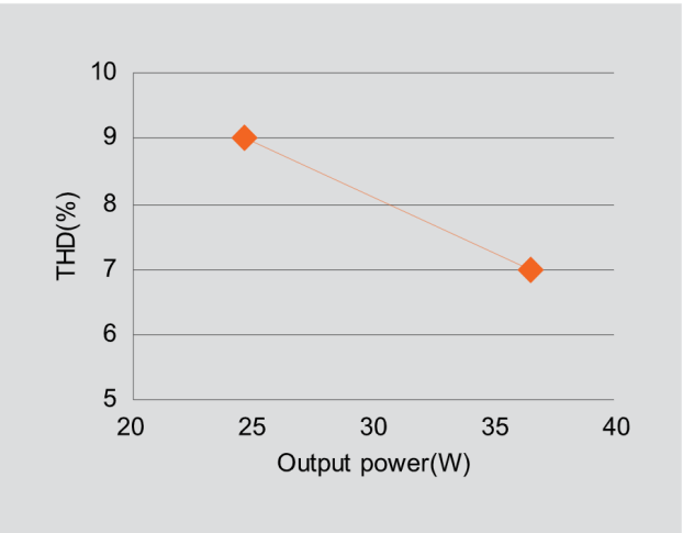
36W 800mA THD
