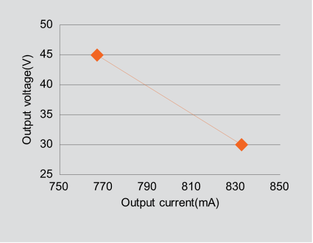
36W 800mA TYPICAL OPERATING WINDOW
