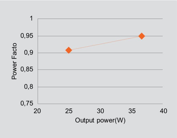
36W 800mA POWER FACTOR
