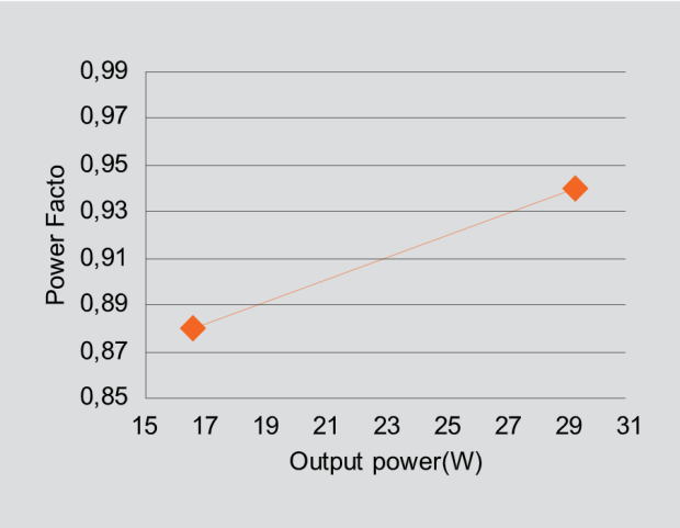
28W POWER FACTOR
