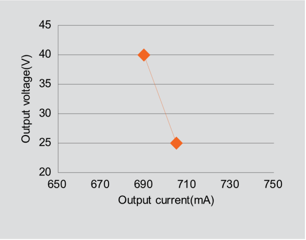
28W TYPICAL OPERATING WINDOW
