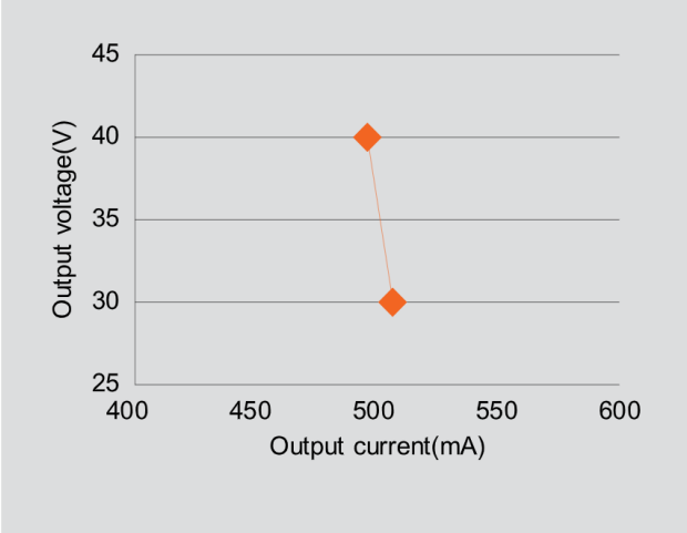
20W TYPICAL OPERATING WINDOW
