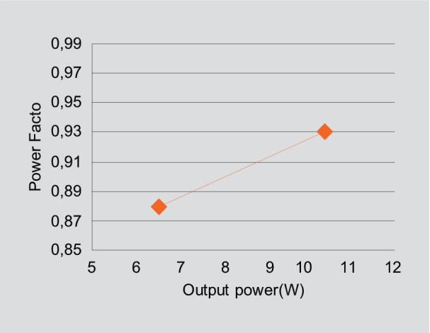
10W 260mA POWER FACTOR
