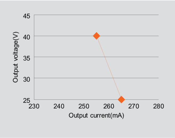
10W 260mA TYPICAL OPERATING WINDOW
