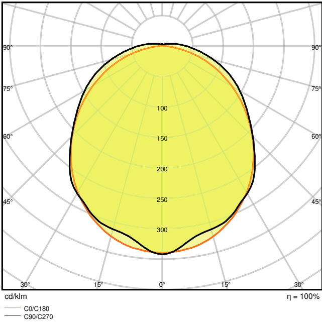
DampProofLED DALI 1500 55W 4000K IP65
