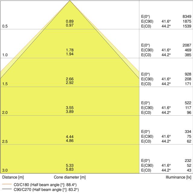
Panel 625 DALI 36W 4000K MP
