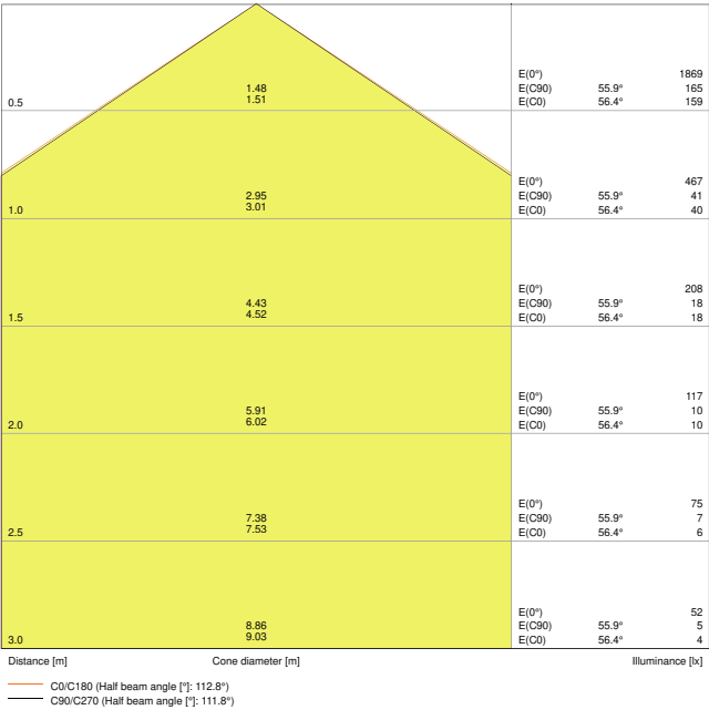
SF BLKH 300 15W3000K BK IP65 LEDV LDT
