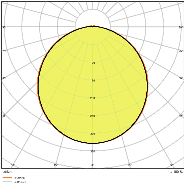
SF BLKH 250 10W4000K WT IP65 LEDV LDT
